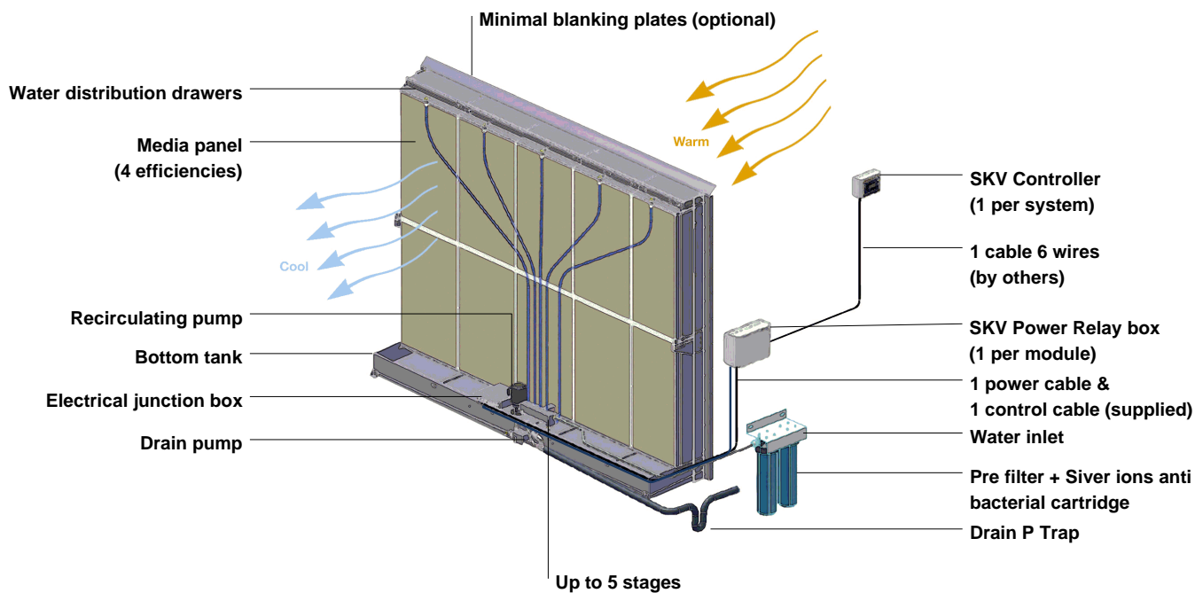
Illustration 1 - Evaporative Media
