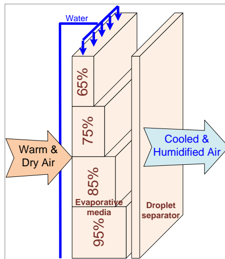
Illustration 1 - Evaporative Media
